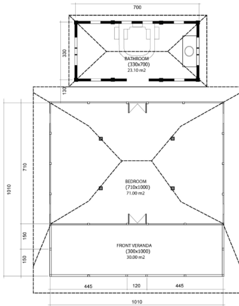
"Kudus" House Floor Plan
