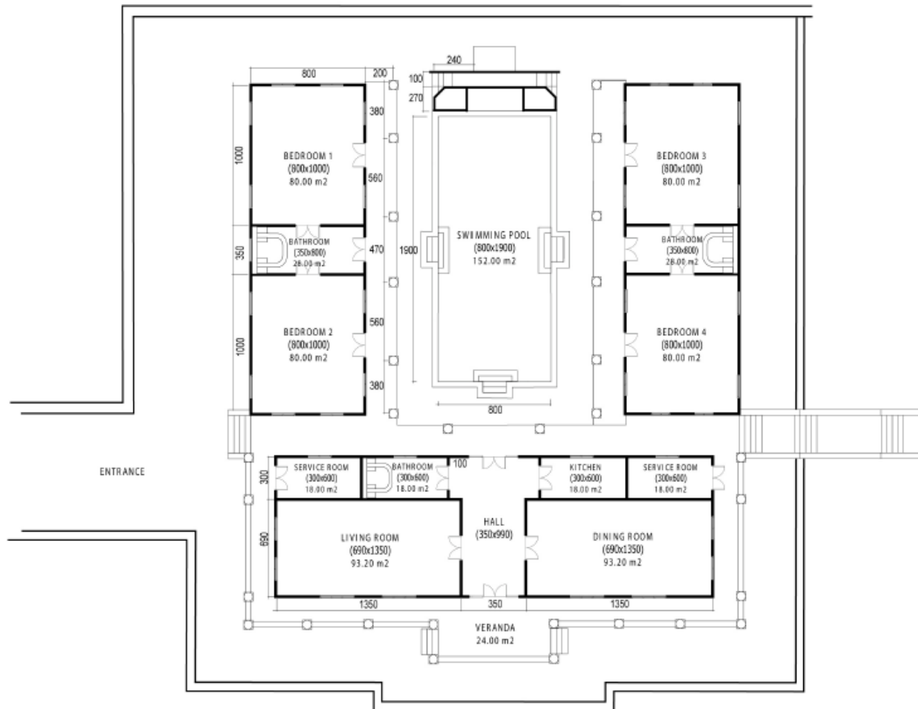
"Old Batavia" Plantation House Floor Plan
